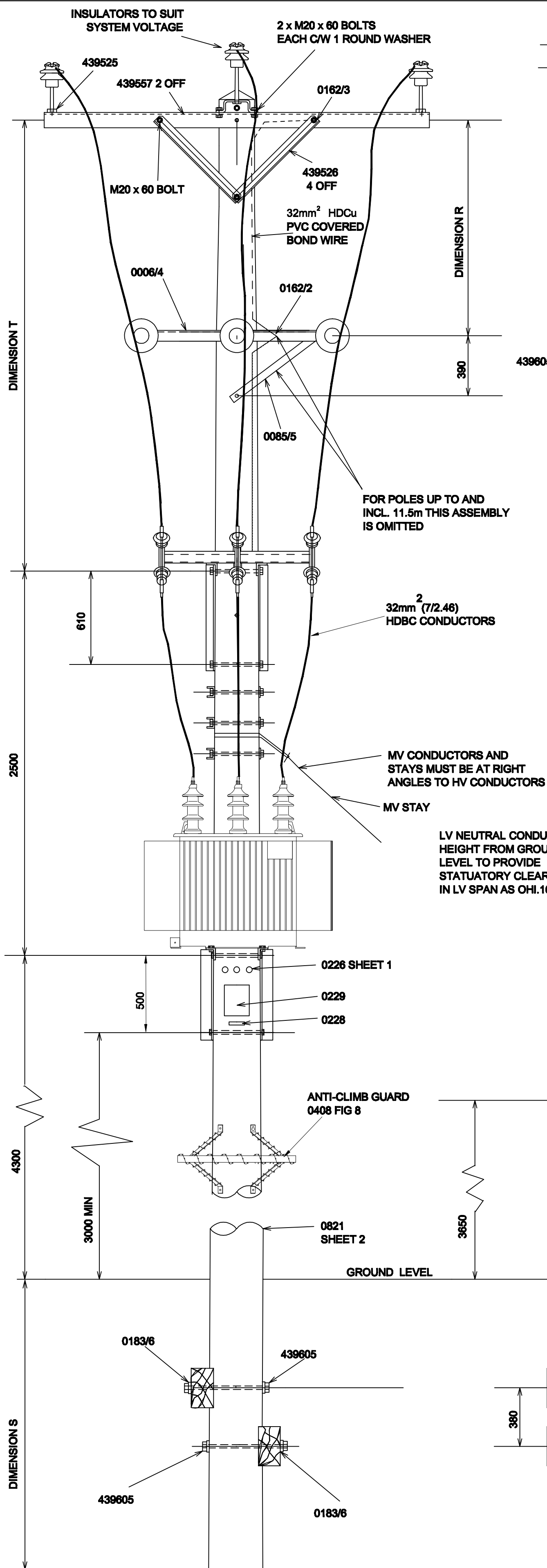
FIG 1 PLATFORM MOUNTED TRANSFORMER IN LINE ARRANGEMENT
